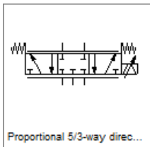
Proportional 5/3-way directional valve
