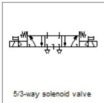
5/3-way solenoid valve
