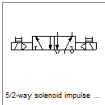
5/2-way solenoid impulse valve
