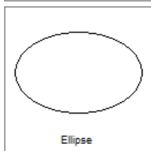
Ellipse
