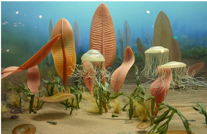
Starohory
