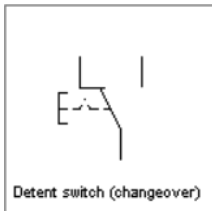
Detent Switch (changeover)
