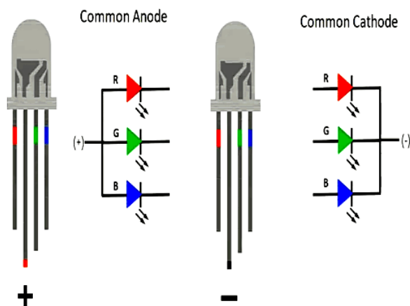
Common Anode Common Cathode Zapojenie RGB LED
