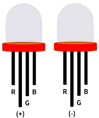
Common Anode (+) Common Cathode (-) Kontakty RGB LED
